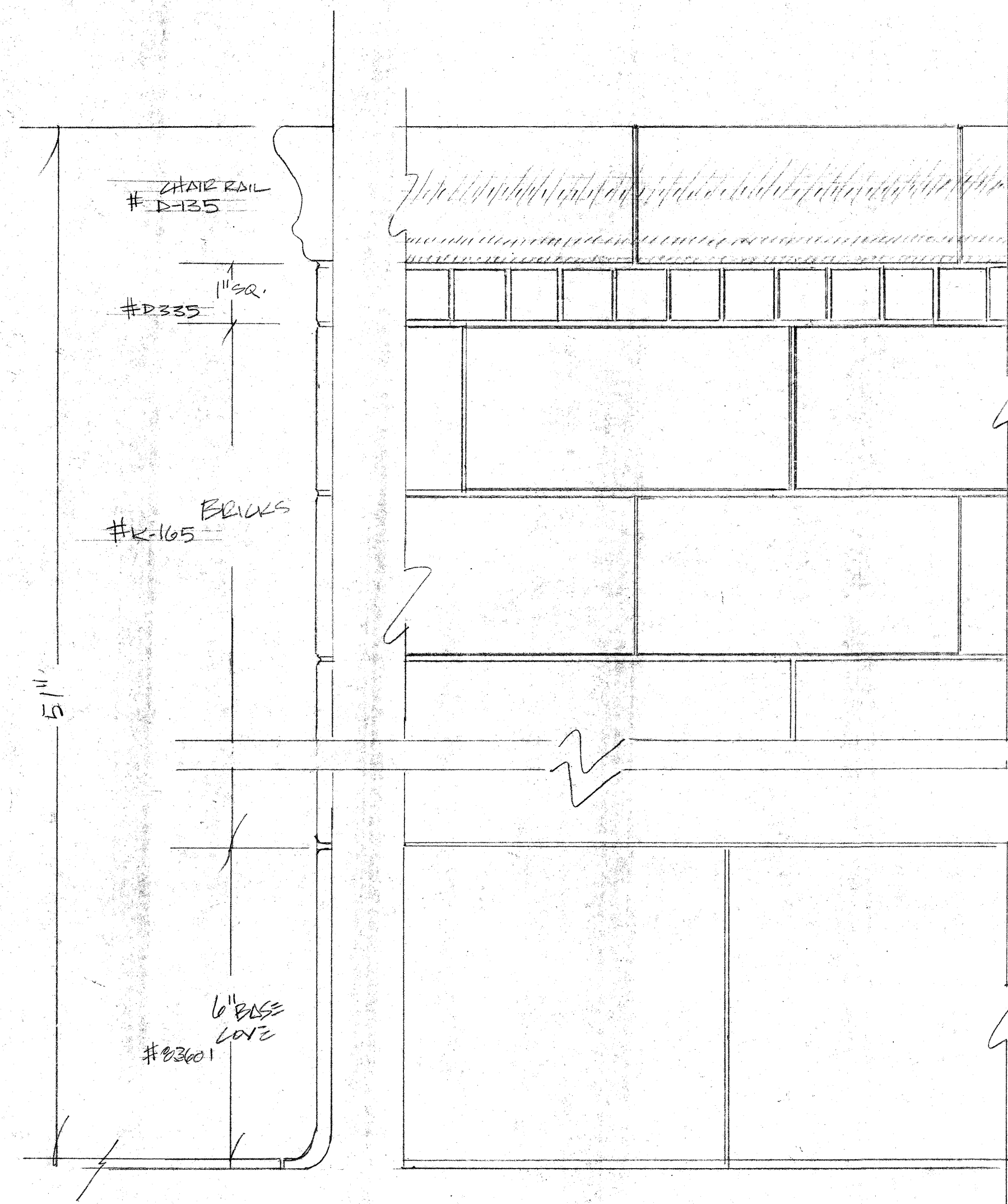
TILE VANSCOTTING DETAIL 1/2" = 1"
